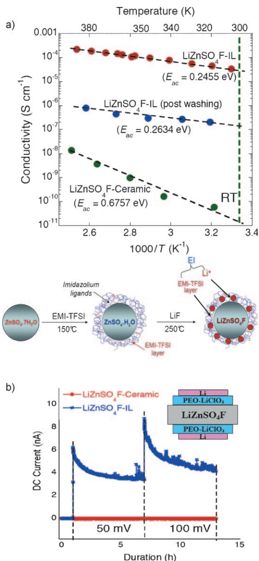
Figure 2. a) AC conductivity of ionically blocking LiZnSO 4 F pellets prepared using ZnSO 4 ·H 2 O precursor made with and without ionic liquid. The presence of a thin layer of ionic liquid (from the precursor) leads to a very high Li-ion room-temperature conductivity of approximately 10 −5 S cm −1 . Even after multiple washings of the sample with ethyl acetate, a permanent layer of ionic liquid remains on LiZnSO 4 F, giving a high conductivity of about 10 −7 S cm −1 . A schematic depiction of the ionic conductivity enhancement caused by the capture of ionic liquid layer around the particles is given (bottom). The “ceramic” LiZnSO 4 F sample, on the other hand, gives a very low conductivity of approximately 10 −11 S cm −1 . The activation energy values ( E ac ) are provided. b) Polarization current measurement of LiZnSO 4 F pellets with and without ionic liquid in a Swagelok cell with Li | PEO | LiZnSO 4 F | PEO | Li configuration (inset; PEO = poly(ethylene oxide)). The current solely involves Li + ion mobility through the LiZnSO 4 F pellet, thus showing that it is a Li + ion conductor. The presence of ionic liquid favors higher Li + ion conductivity.
